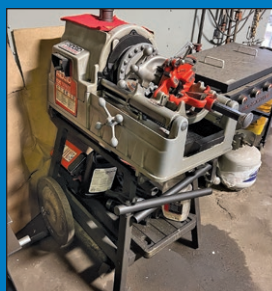
Ridgid 535 Pipe Threader
