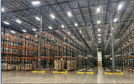
(530+) Sections 42" x 8' W x 33' H Pallet Rack
