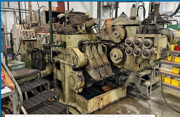
(7) National Cold Headers, Models 1000, S-2, 89, 56 and 34
