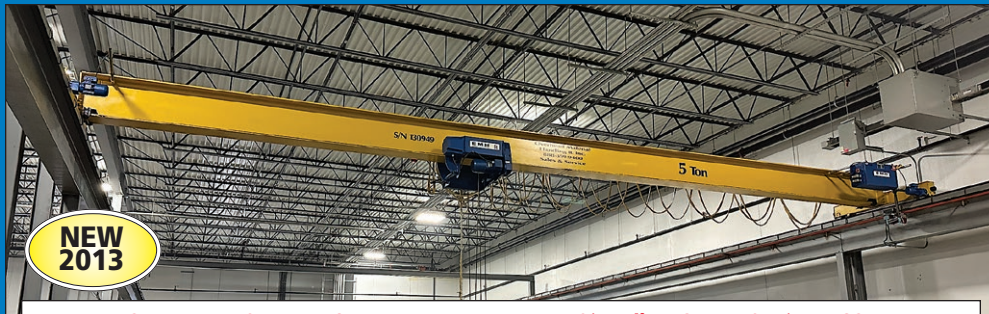
5-Ton x 50' Approx. Span x 125' Approx. Long Free-Standing Crane System (2013)
