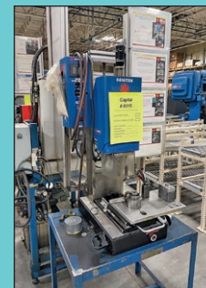
(6) Sonitek Model S10 Heat Staking Presses
