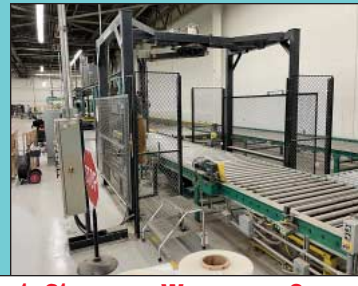
Automated Palletizing and Wrapping Line w/ Robot, Strapper, Wrappers, Conveyor and Palletizer
