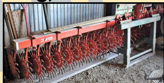
Yetter 3415 Rotary Hoe, 15' wide, 3 point
