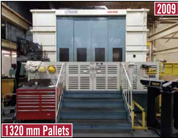
NIIGATA HN130D CNC Horizontal Machining Center
